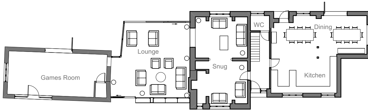
The Oast - Ground Floor
