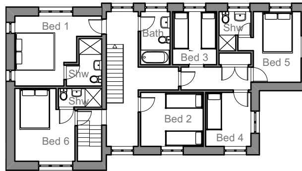
The Oast - First Floor
